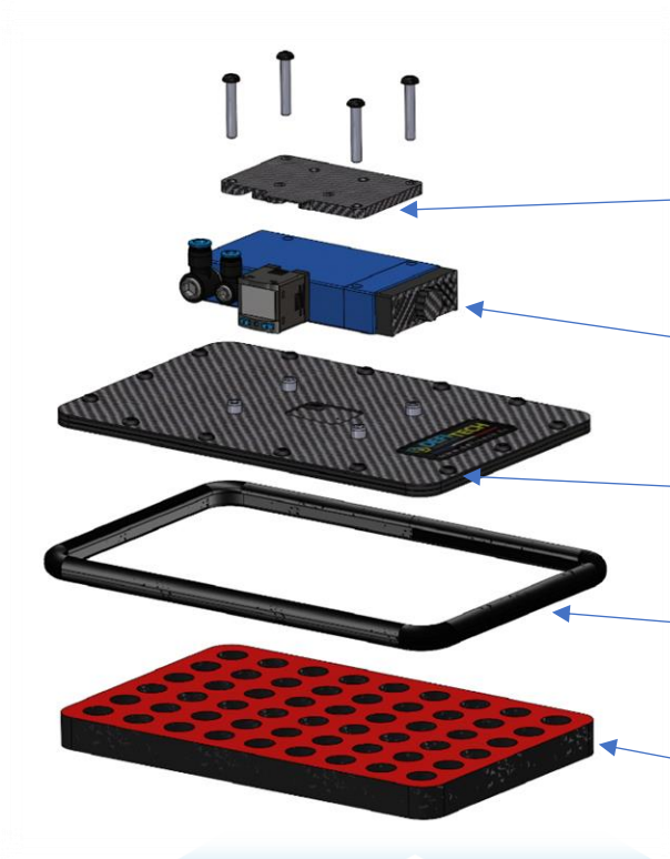
Robot attachment
